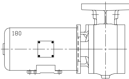
Horizontal Mount NEMA Motor
